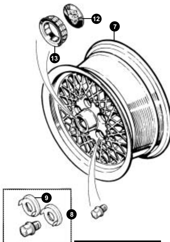
Sportspack Alloy
